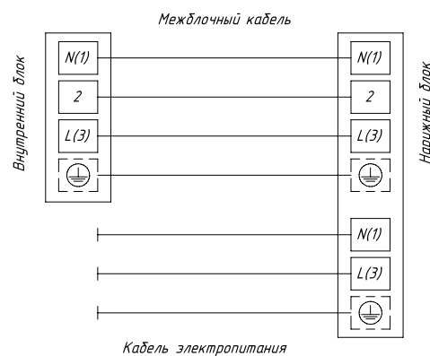
RAC-I-ON55HP.D01/U RAC-I-ON70HP.D01/U
